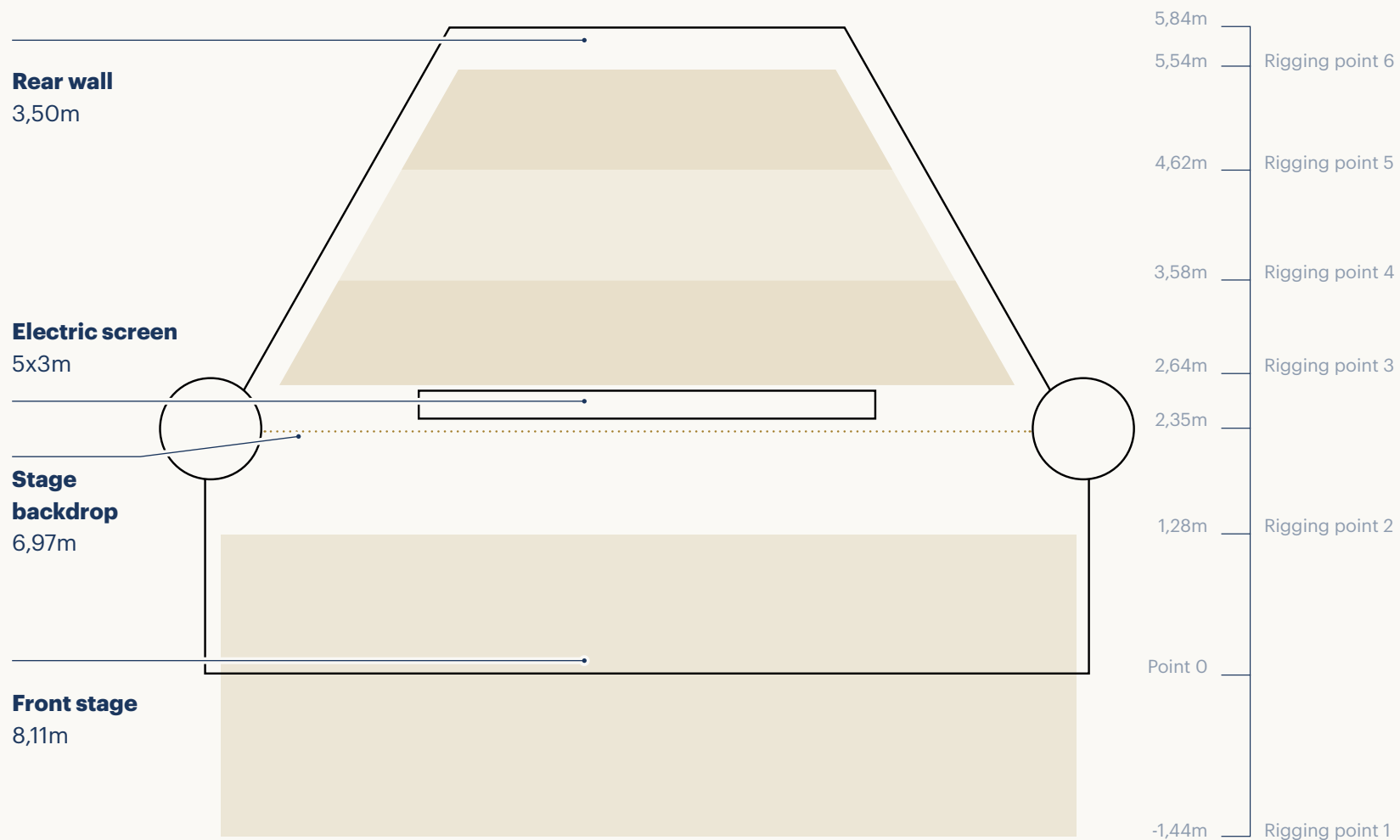
STAGE GRID
